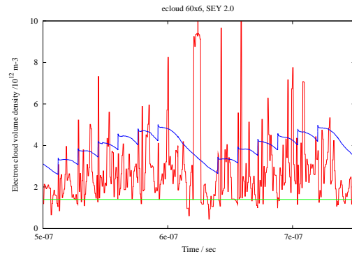
Figure 13: Detailed view of the simulated central volume density of the electron cloud for 60x6 bunches (red line). The green line corresponds to the threshold density of 1.4 \cdot 10^{12} \text{ m}^{-3} . Furthermore the total number of electrons in the cloud is shown in arbitrary units (blue line).
